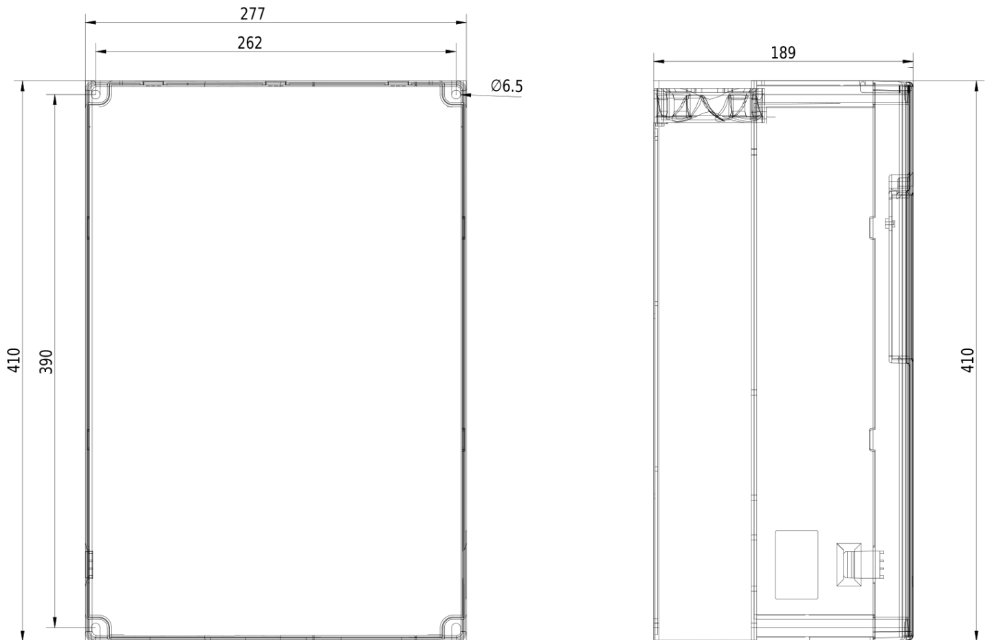
Dimensional drawing V810 - 22kW 4T0220
