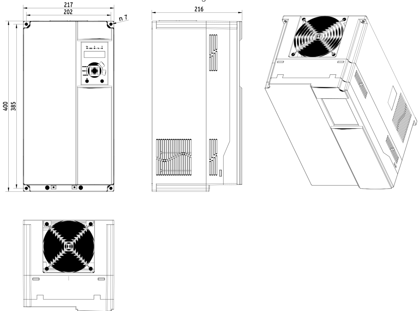
Dimensional drawing V900 - 45kW 4T0450
